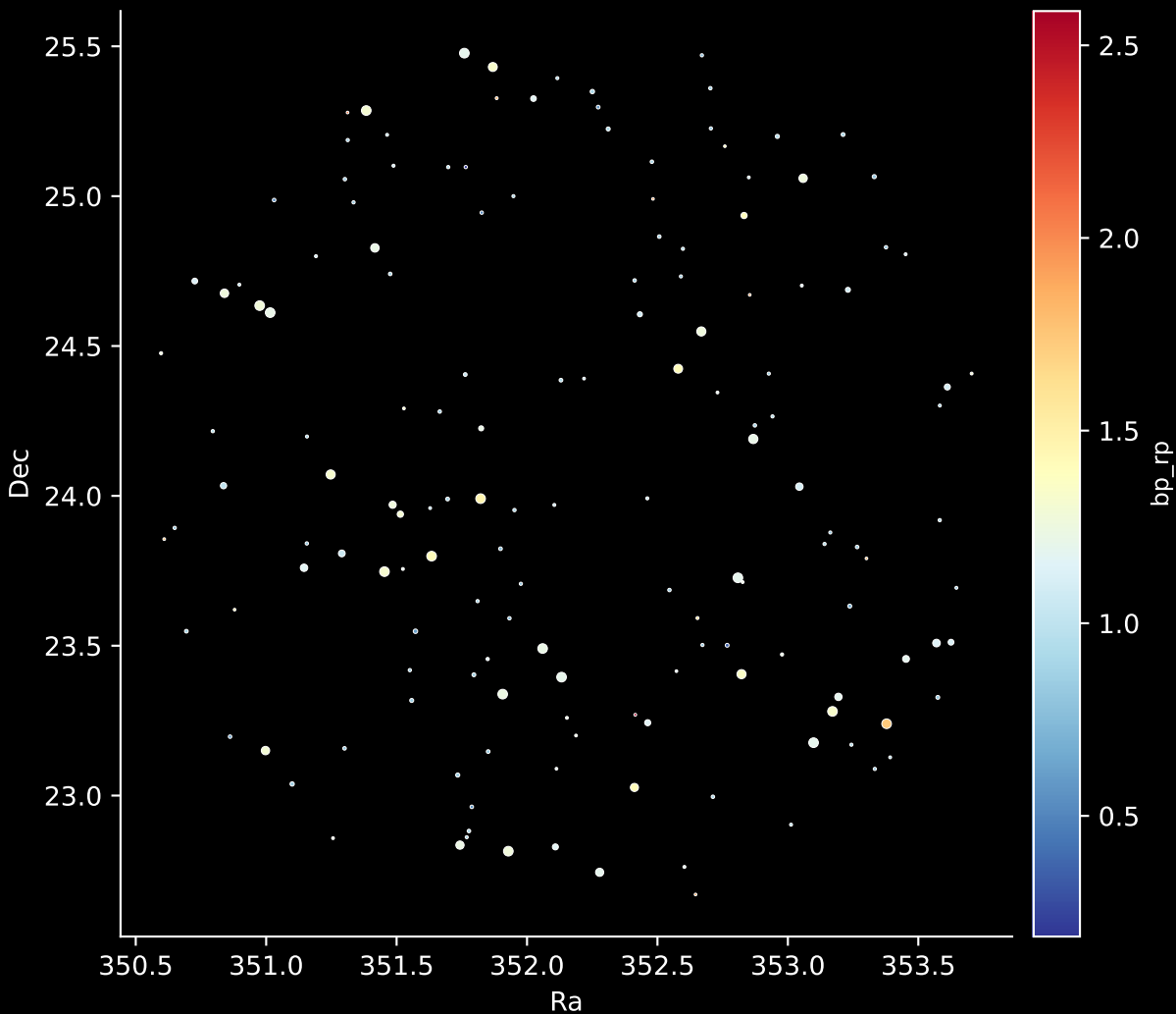
APOGEE DR17 Field: [044+37_MGA] Stars: 153
