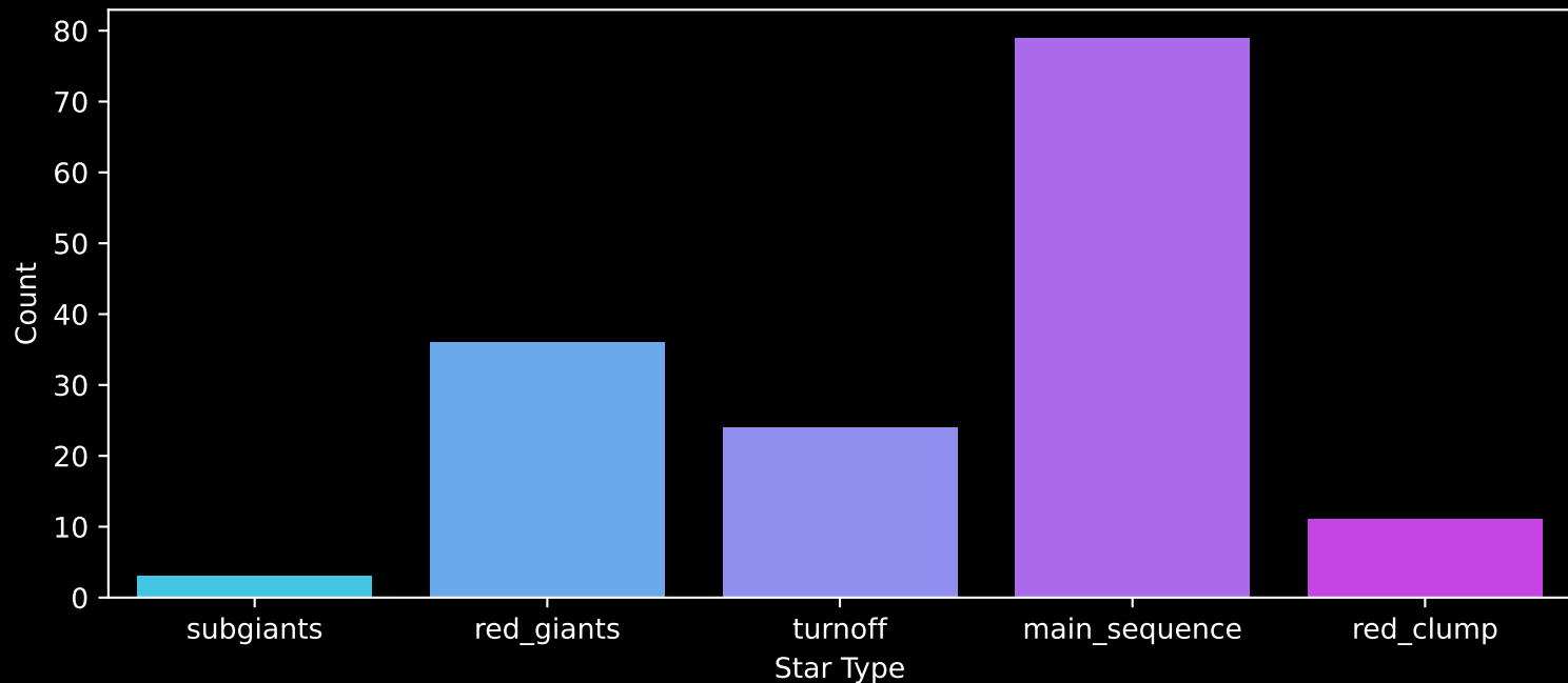
APOGEE DR17 Field: [044+37_MGA] Count plot of Star Type
