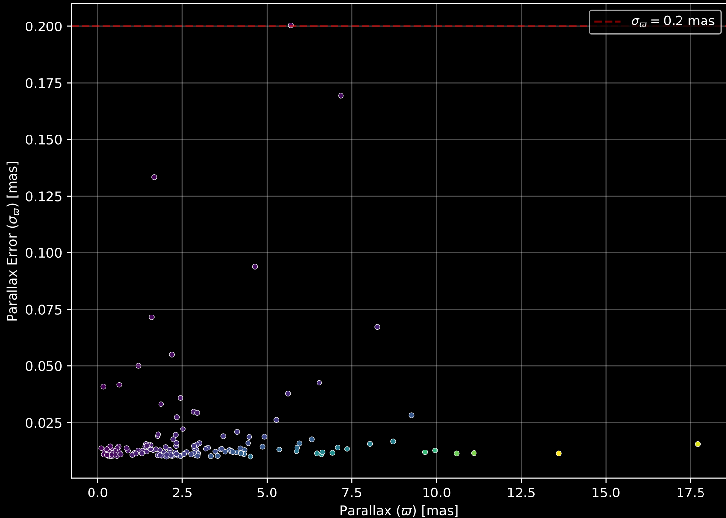
APOGEE DR17 Field: [044+37_MGA] Parallax Quality (n= 153)
