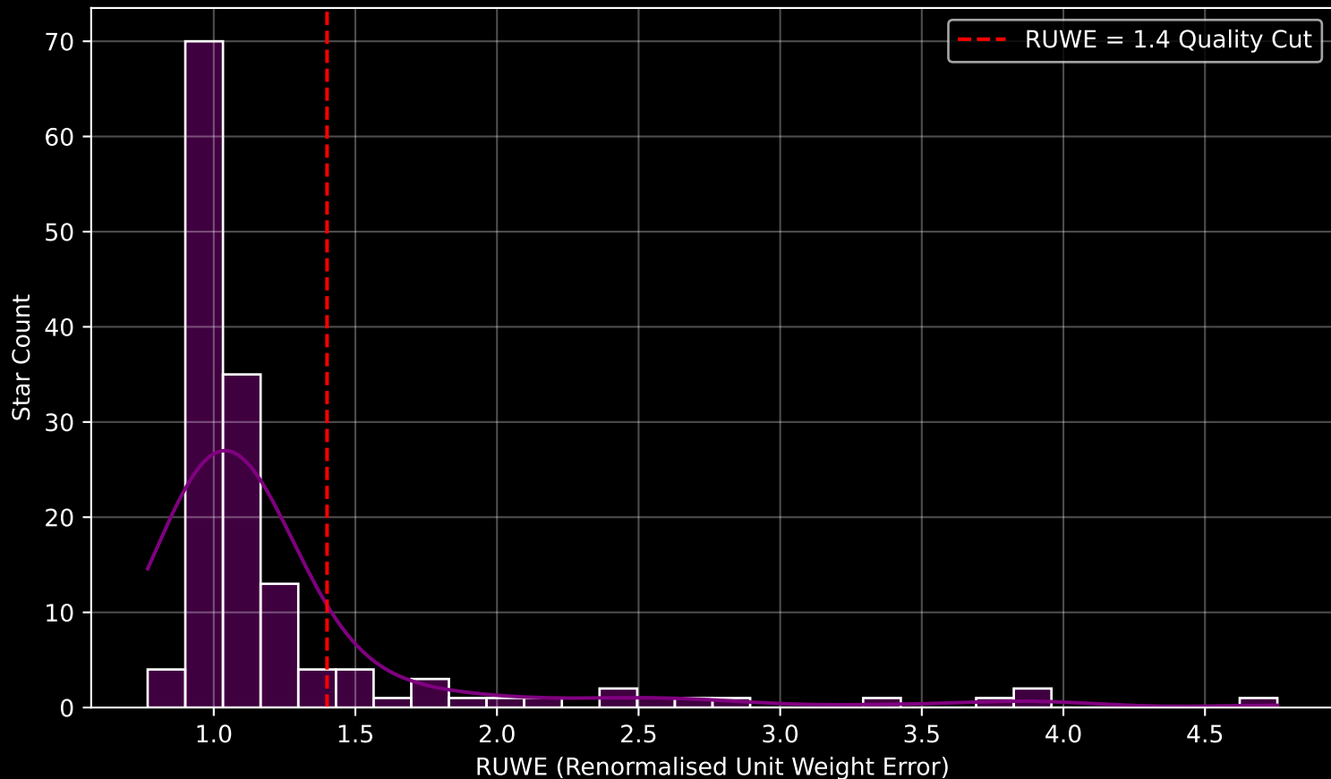
GAPOGEE DR17 Field [044+37_MGA] RUWE Distribution (n= 147)
