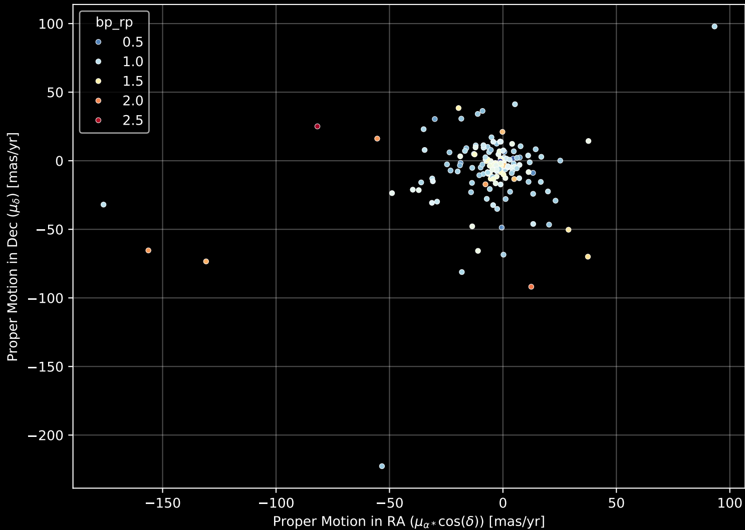
APOGEE DR17 Field: [044+37_MGA] Proper Motion Diagram (n= 153)
